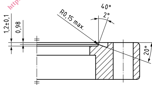
Figure 2 — Knife-edge detail
