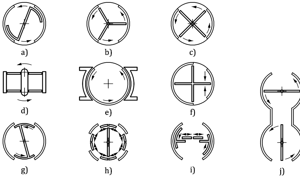
Figure 1 — Revolving doorsets
