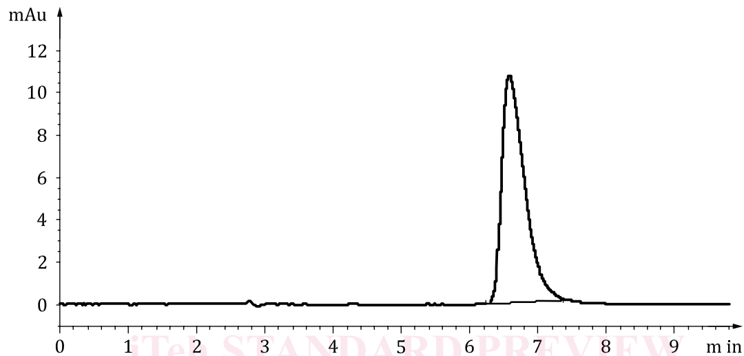
Figure A.1 — HPLC chromatogram of standard picric acid
