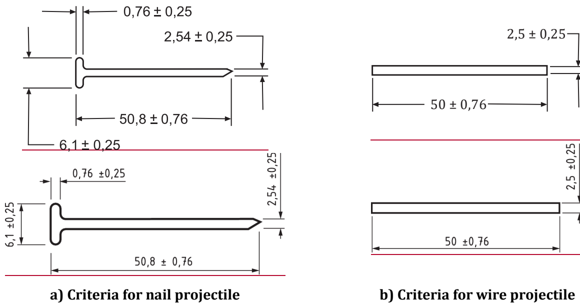
Figure 1 — Test projectile iTeh STANDARD PREVIEW (standards.iteh.ai)
