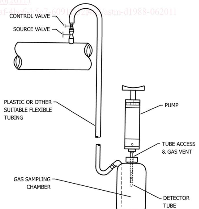
FIG. 1 Apparatus Schematic
