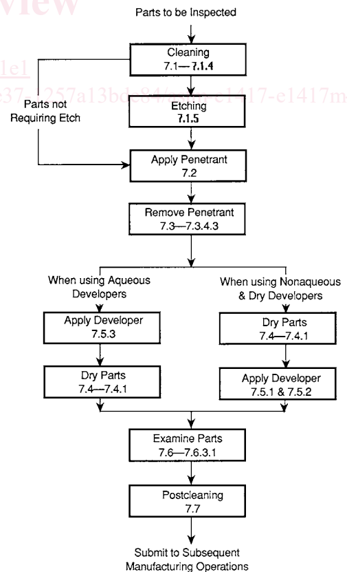
FIG. 1 Process Flow Chart
