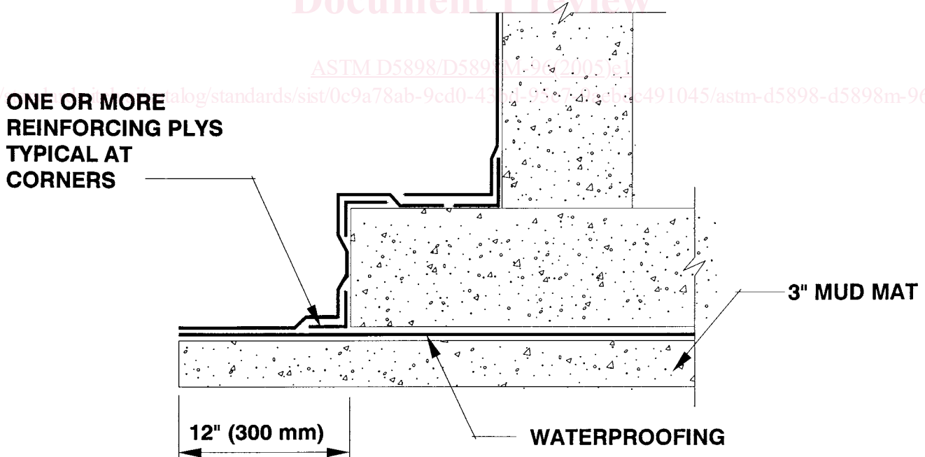
FIG. 3 Slab with Mud Mat
