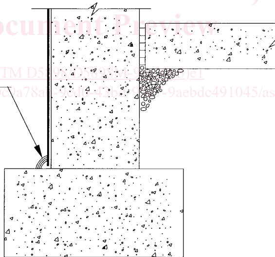
FIG. 5 Footing with Raised Slab
