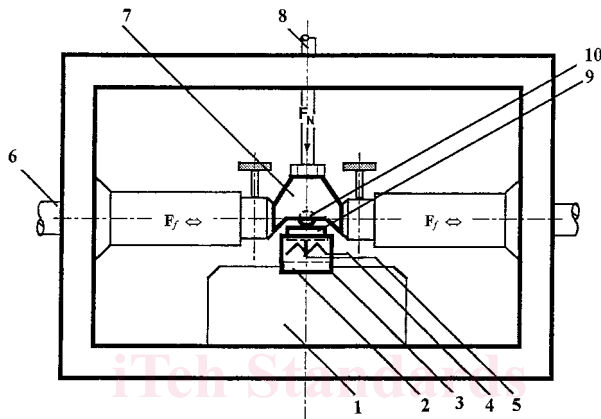
FIG. 2 Test Chamber
