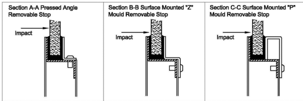
FIG. 2 Test Assembly Door Elevation #2 Location of Strike Points Described in Table 2
