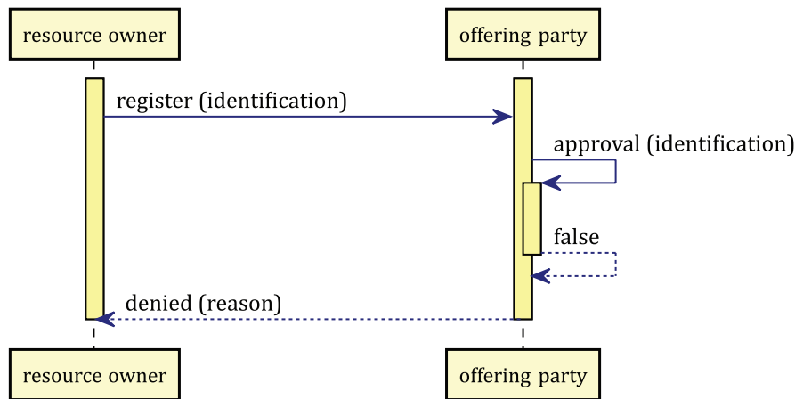
Figure 6 — Rejecting registration of the resource owner at the offering party (standards.iteh.ai)
