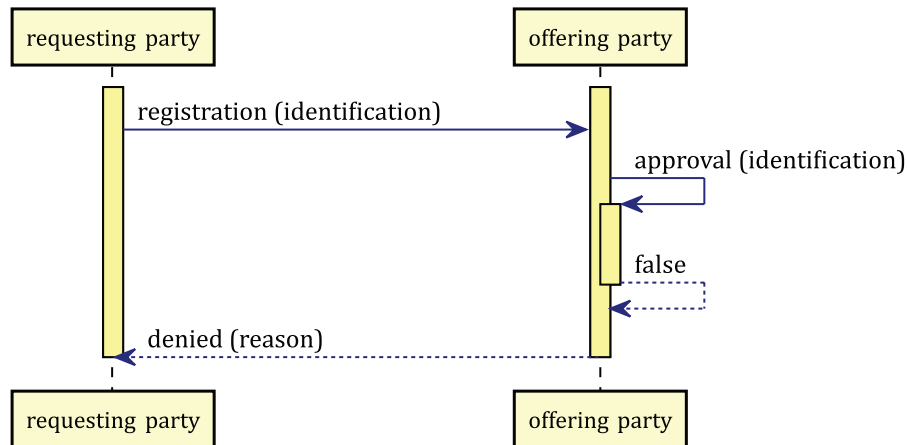
Figure 4 — Registration of a requesting party is rejected by the offering party
