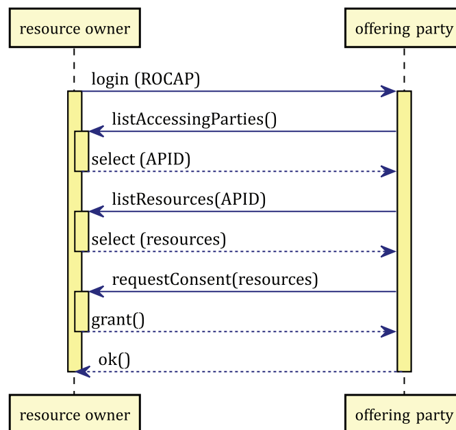
Figure 8 — Implicitly granting access to resources
