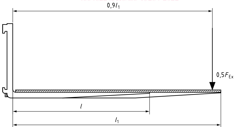
Figure 2 — Test/design load for open-section fork arms
