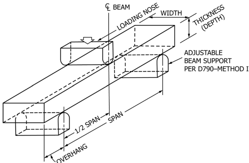
FIG. 1 Type B Specimen Geometry and Loading
