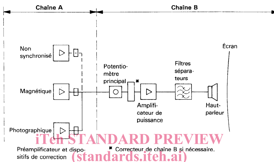
Figure 1 — Système complet de reproduction sonore de salle https://standards.iteh.ai/catalog/standards/sist/c21359ed-9717-4c97-b85e-3bc735d62929/iso-2969-1987
