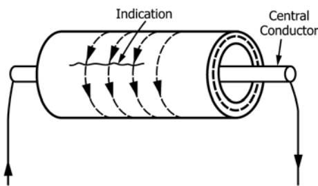
FIG. 4 Circular Magnetization, Current Through a Conductor
