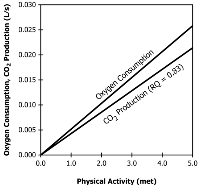
FIG. 1 CO_2 Generation and Oxygen Consumption as a Function of Physical Activity
