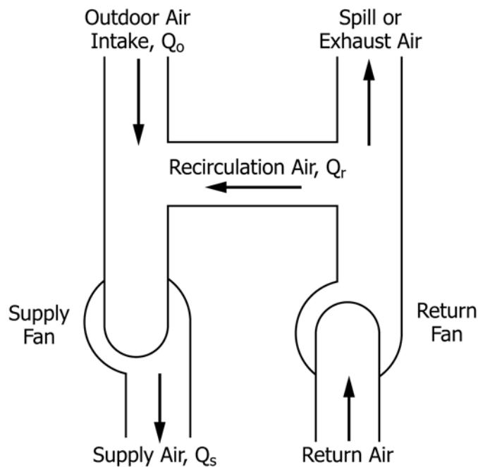
FIG. 3 Air Handling System Schematic
