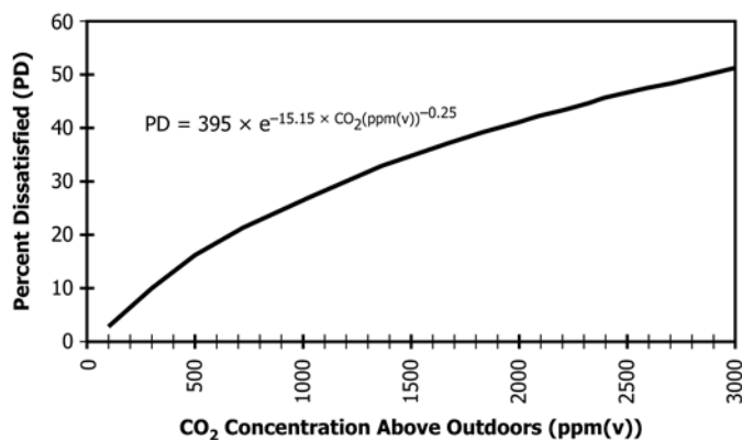
FIG. 2 Percent of Visitors Dissatisfied as a Function of CO 2 Concentration (8)
