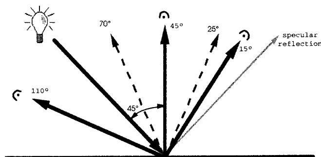
NOTE 1—Solid lines indicate preferred angles. FIG. 2 Diagram of Aspect Angles
