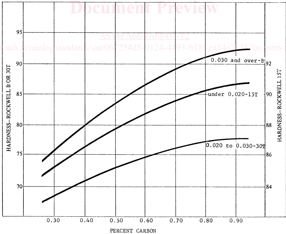
FIG. 2 Approximate Relationship Between Carbon Designations and the Maximum Hardness Limit of Spheroidized Annealed Cold Rolled High Carbon Steel Strip
