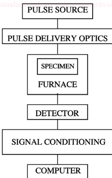
FIG. 3 Block Diagram of a Flash System
