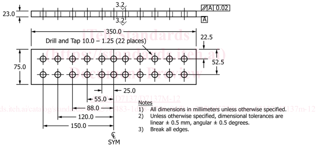
FIG. 4 Support Fixture Base Plate (SI Version)
