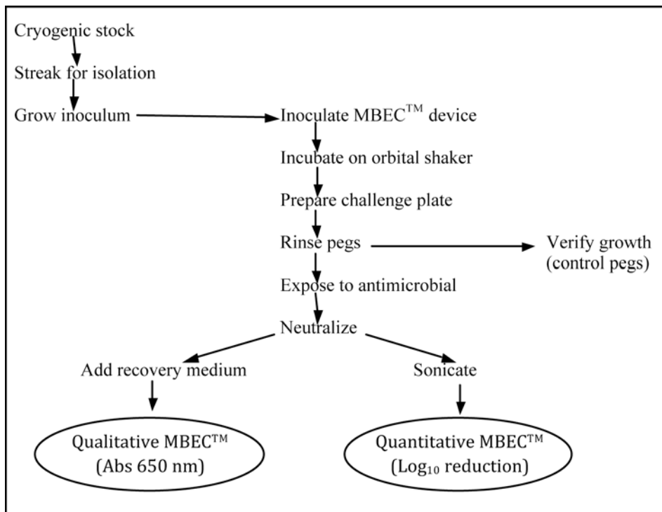
FIG. 2 3 A Flow Diagram Representing the MBEC Assay for Disinfectant Testing
