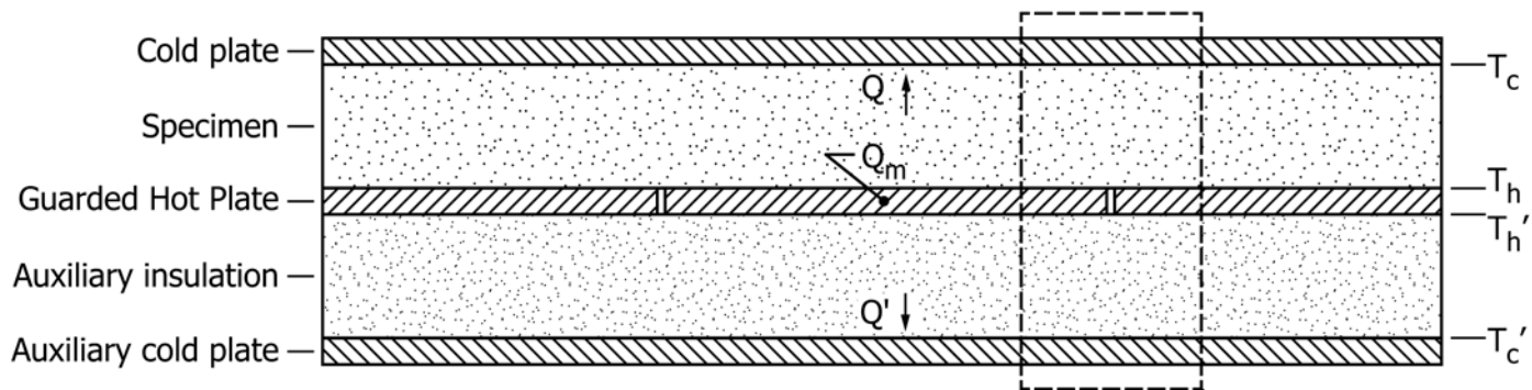
Single - Sided Mode of Operation
