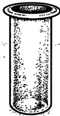
C. Glass Insert (height 58 mm, diameter at bottom 16 mm and diameter of flared end at the top 20 mm)
