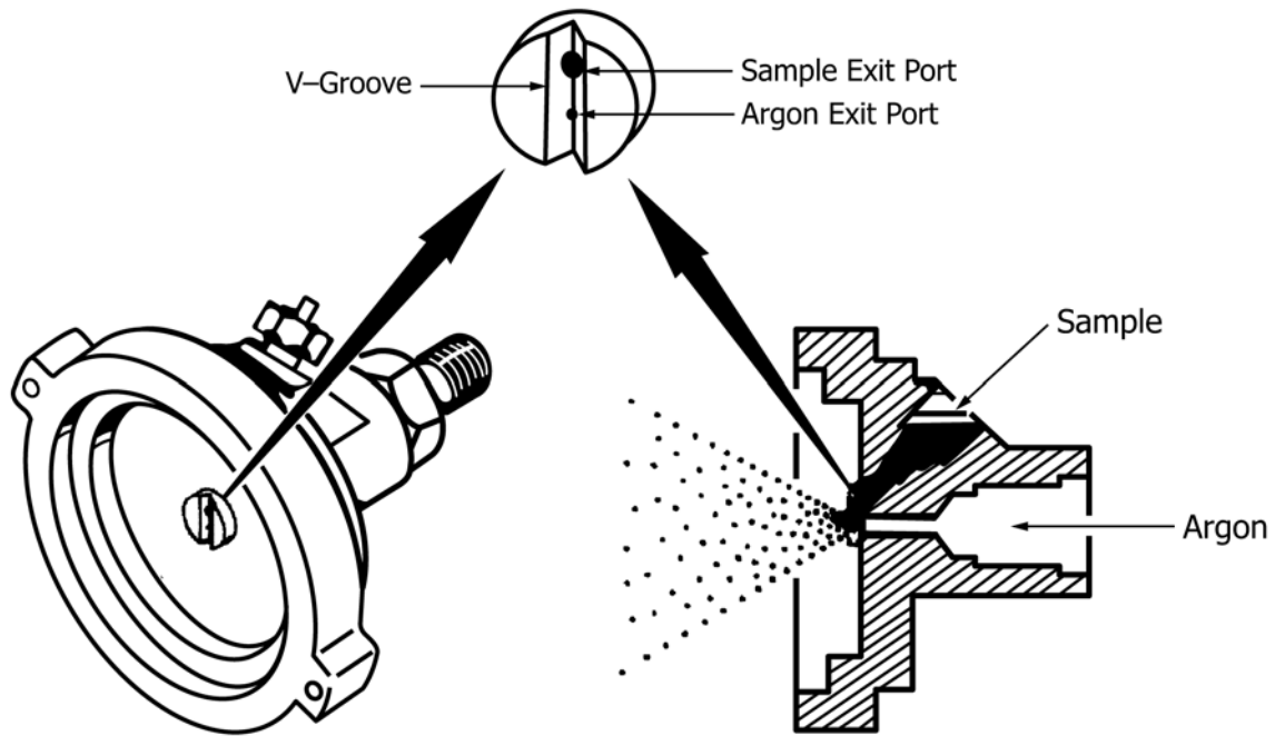
FIG. 6 Babington-Type Nebulizer 4
