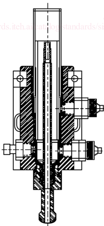
FIG. 9 Demountable Torch 9
