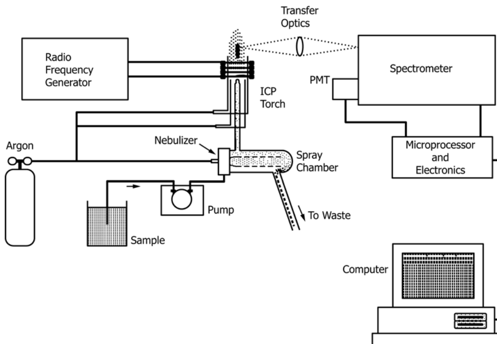
FIG. 1 Components of Inductively Coupled Plasma 4
