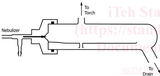
FIG. 7 Spray Chamber 4
