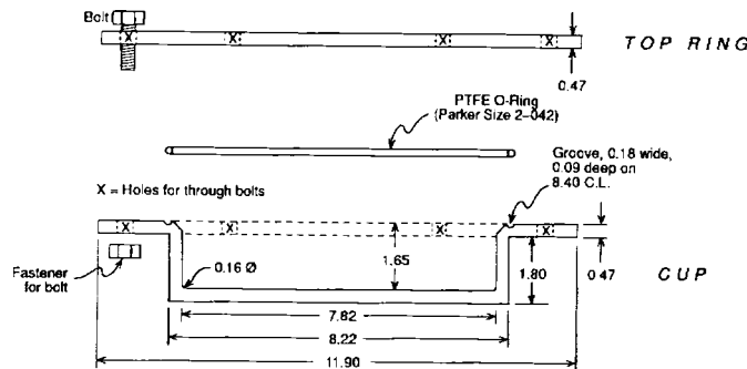
NOTE—Dimensions in centimetres. FIG. 1 ASTM Permeation Cup
