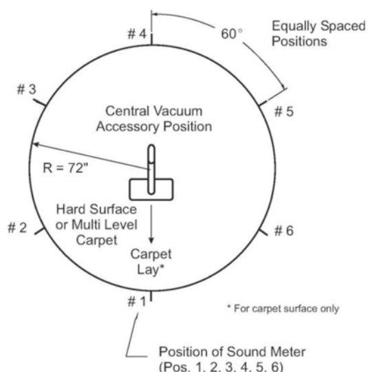
FIG. 4 Sound Test Pattern for CV Accessories
