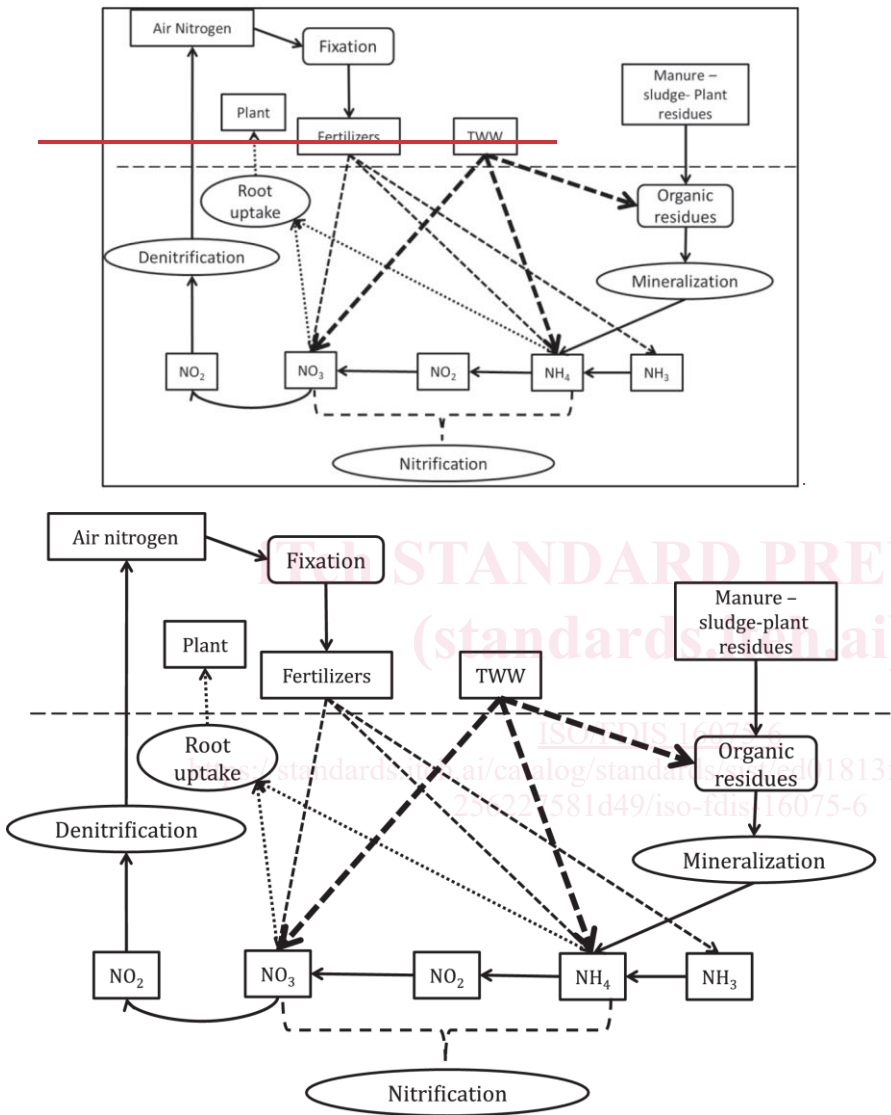
Figure 1 — Nitrogen cycle in the soil
