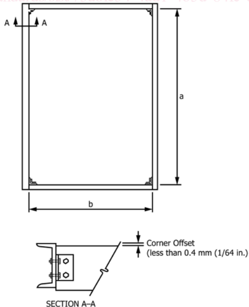
FIG. A1.1 Structural Support System
