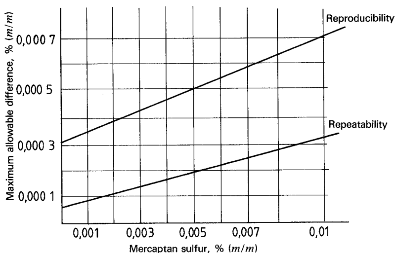
Figure 2 — Precision curves for mercaptan sulfur in gasolines, kerosines, aviation turbine fuels and distillate fuels
