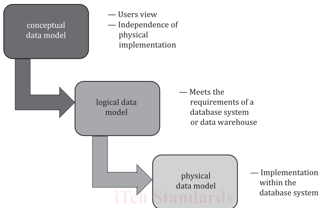
Figure 1 — Levels of data-oriented modelling
