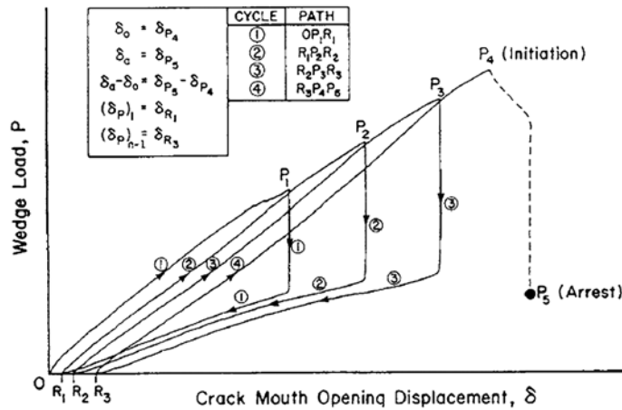
FIG. 8 Wedge-Force Versus Crack-Mouth-Opening-Displacement Record for a Specimen Tested Using Cyclic Loading Techniques, that Displayed Rapid Run-Arrest Fracturing on the Fourth Loading Cycle
