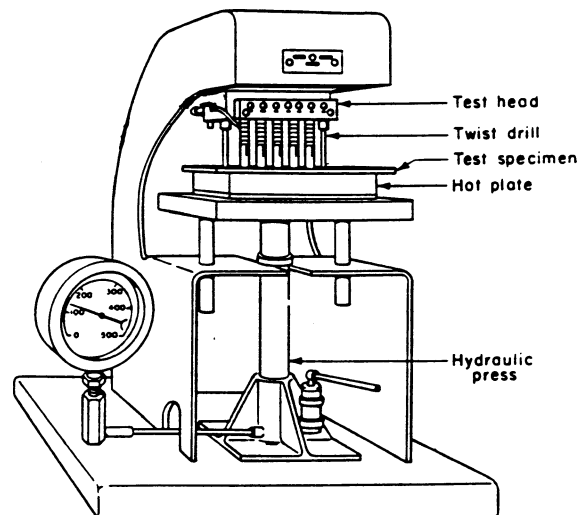
FIG. 1 Apparatus of Surface Insulation Resistivity Measurement
