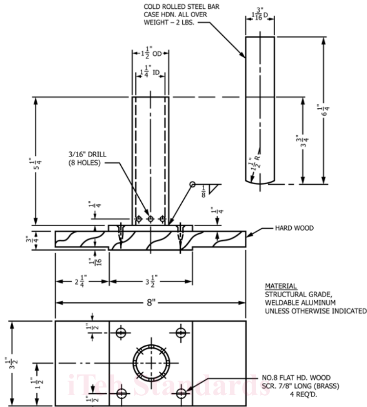
FIG. 2 Drop Hammer for Cross-Brick Couplets
