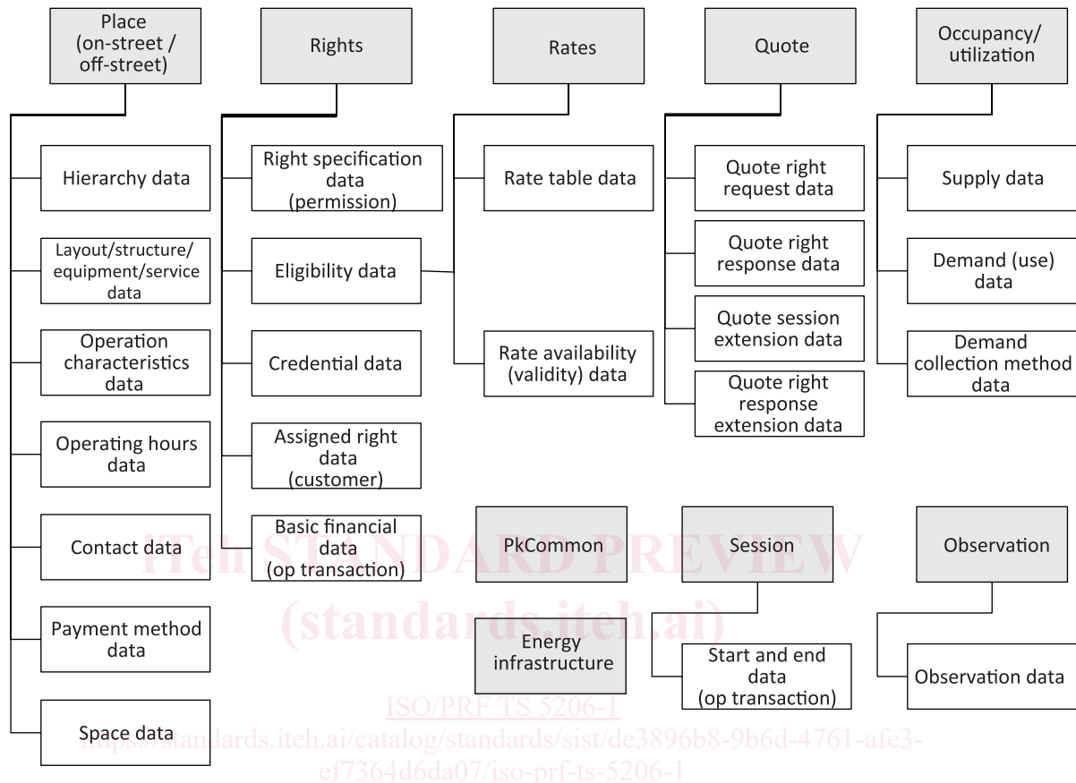
Figure 1 — Data domains
