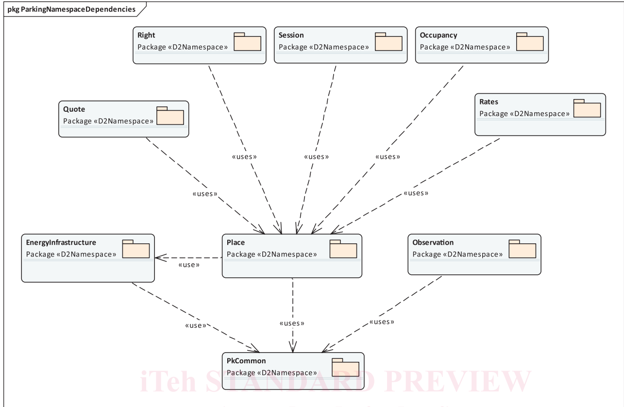
Figure 2 — Namespace dependencies
