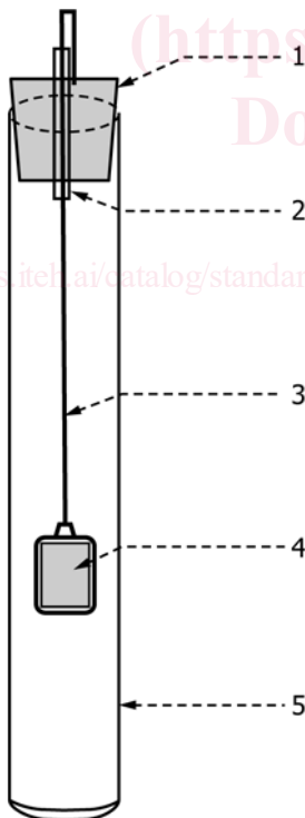
FIG. 2 Silver Strip Suspension Assembly (Procedure A)
