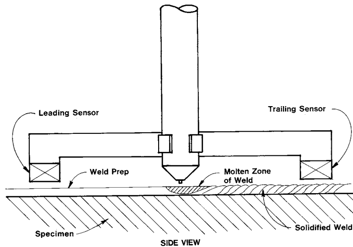
FIG. 4 Moving Sensor Configuration with Sensor Position Fixed Relative to Weld Head
