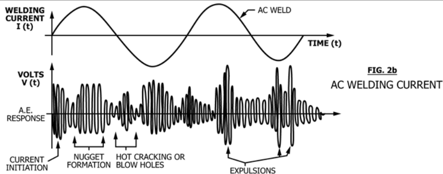
FIG. 2 Typical AE Response Signals During Current Flow
