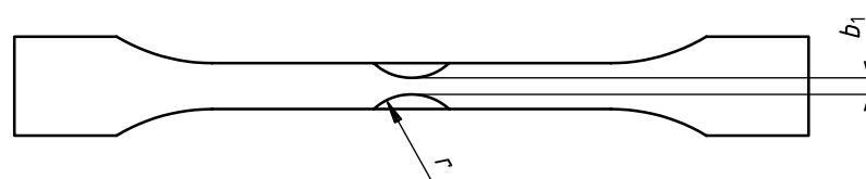
Figure 1 — Details of the ISO 20753/CWx3 small tensile specimen
