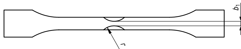
Figure 1 — Details of the ISO 20753/CWx3 small tensile specimen
