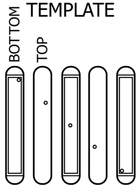
FIG. 2 Method of Sampling Lead by Drilling
