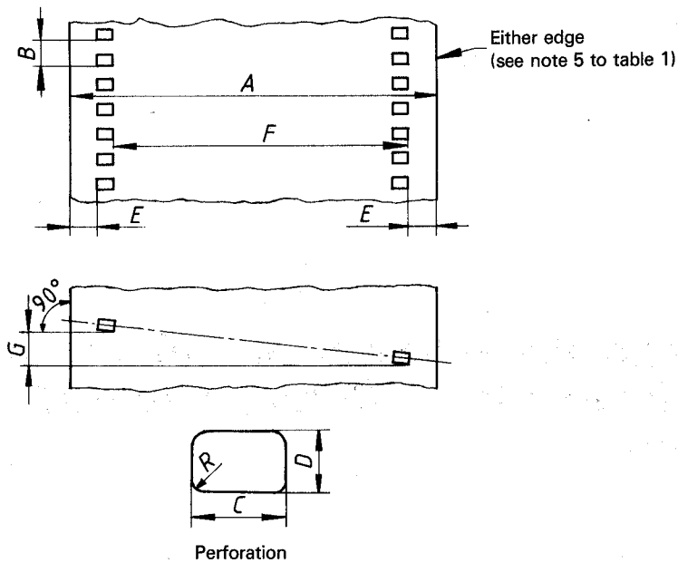
Figure — 65 mm and 70 mm unexposed film
