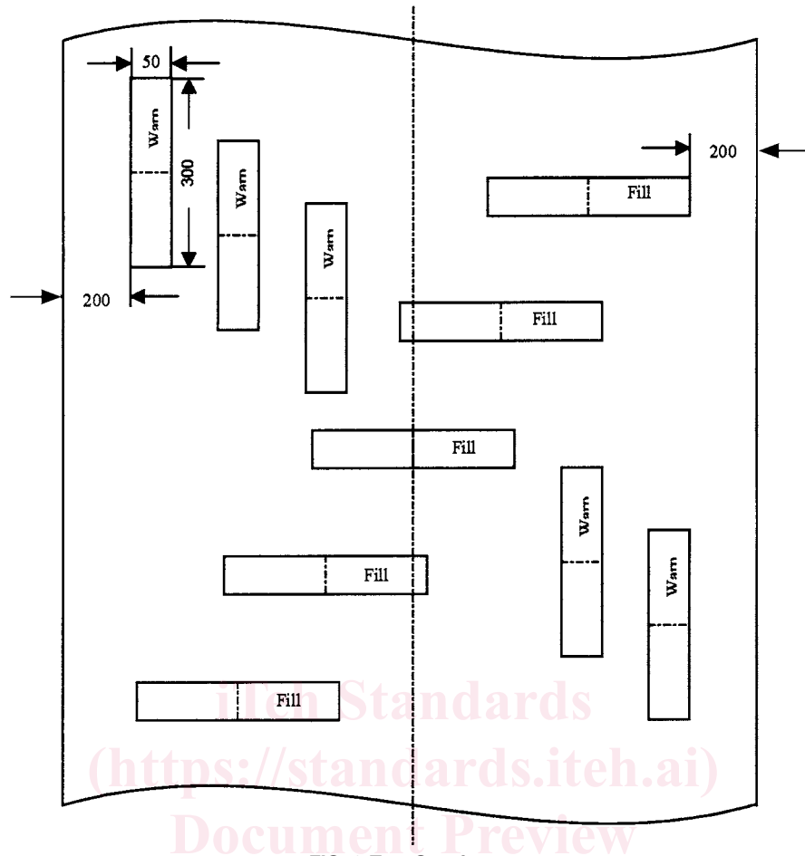
FIG. 2 Test Specimens
