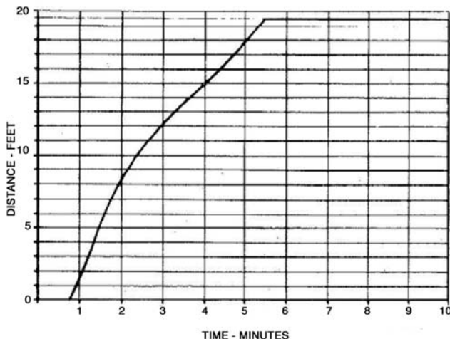
FIG. 8-7 Representative Time-Distance Curve for Flame Spread of Red Oak
