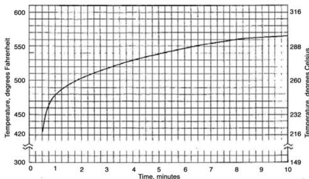
FIG. 7.6 Representative Time-Temperature Curve for Preheat Temperatures
