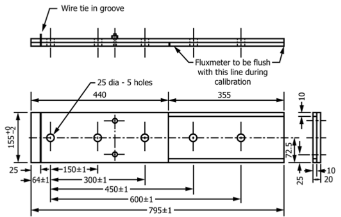
NOTE 1—All dimensions are in millimetres.
