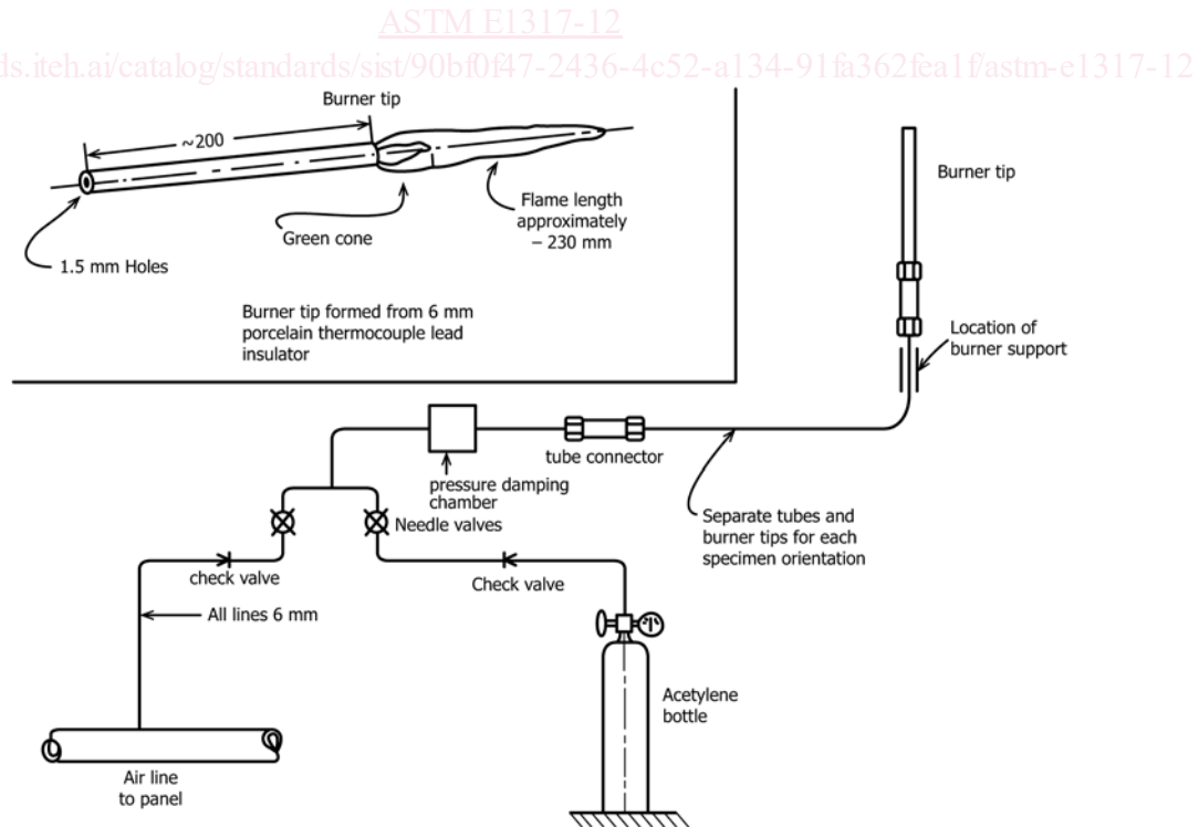
FIG. 8 Pilot Burner Details and Connections
