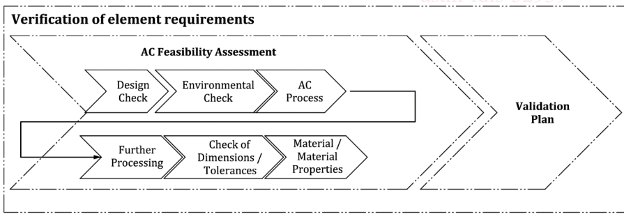
Figure 1 — Steps involved in verification of AC element requirement
