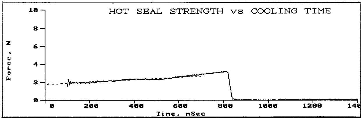
FIG. 2 Cooling Curve
