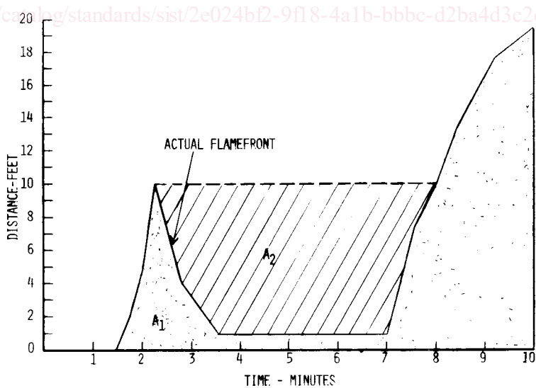
FIG. 11 Example of Time-Distance Relationship with Flame Front Recession (Total Area, A_T = A_1 + A_2 )
