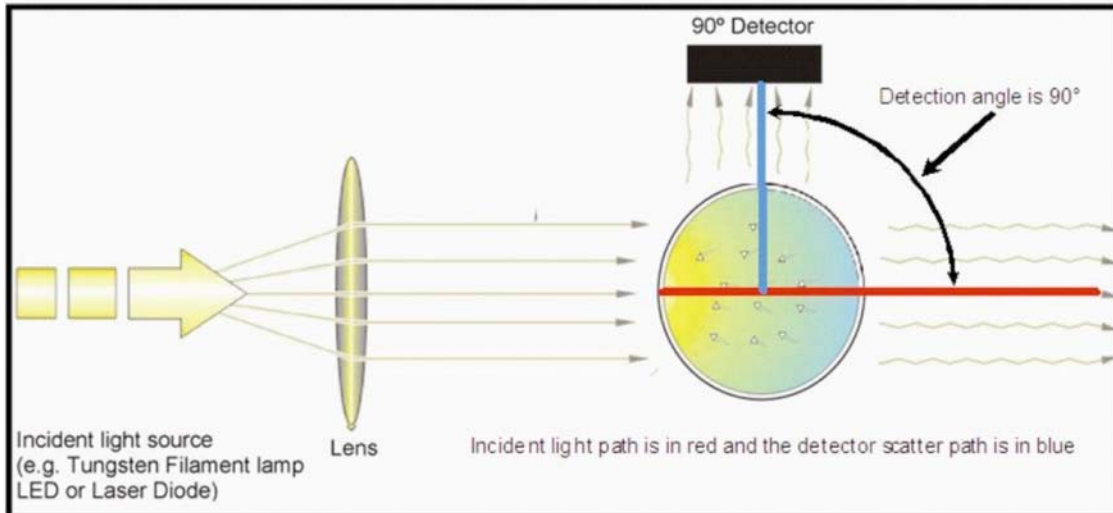
FIG. 1 Photoelectric Nephelometer
