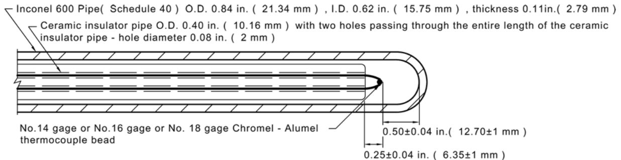
FIG. 2 Thermocouple Assembly
