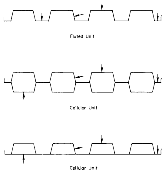
FIG.-2 3 Typical Location of Thermocouples
