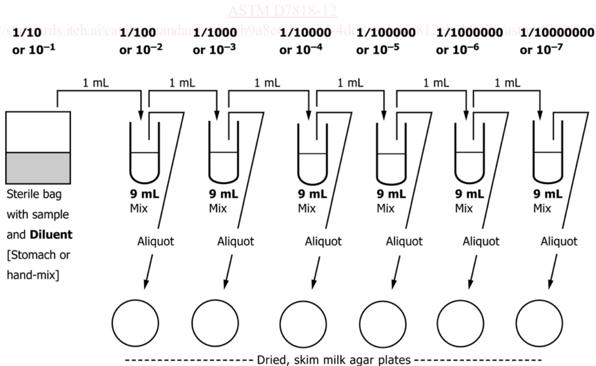
FIG. 1 Plating
